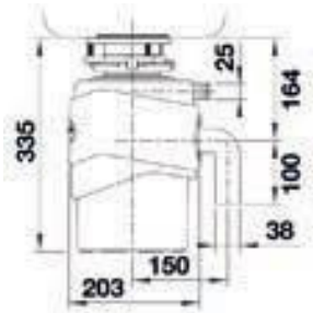
FWD overflow connection
